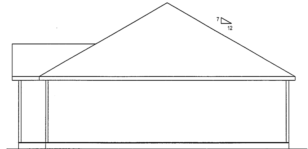
RIGHT VIEW
