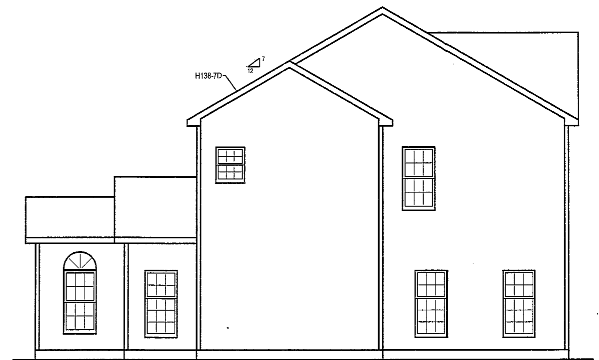
LEFT VIEW
