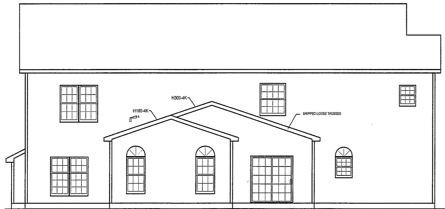
REAR VIEW
