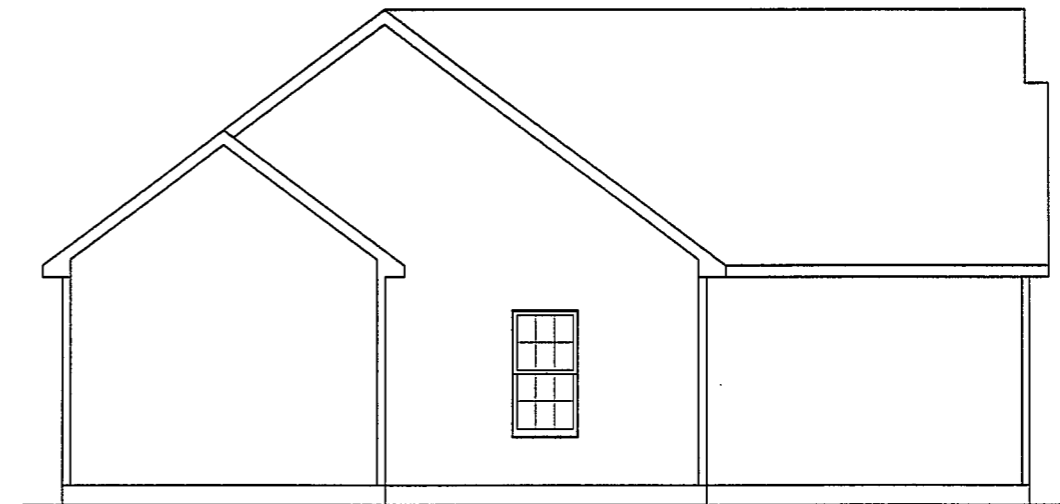
LEFT VIEW
