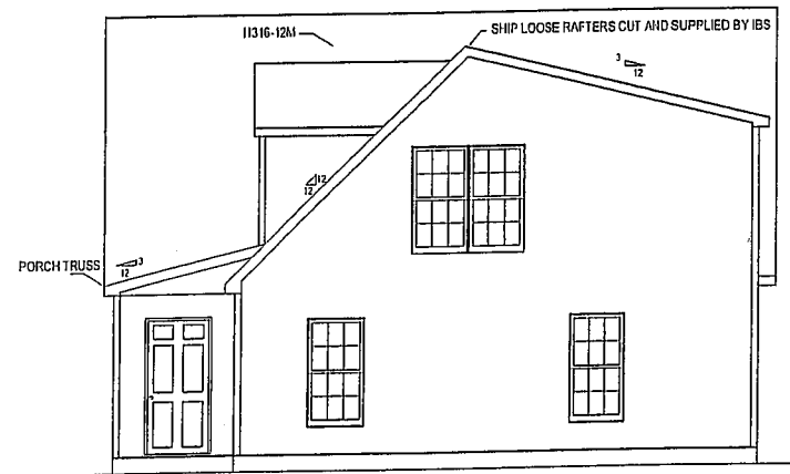
RIGHT VIEW
