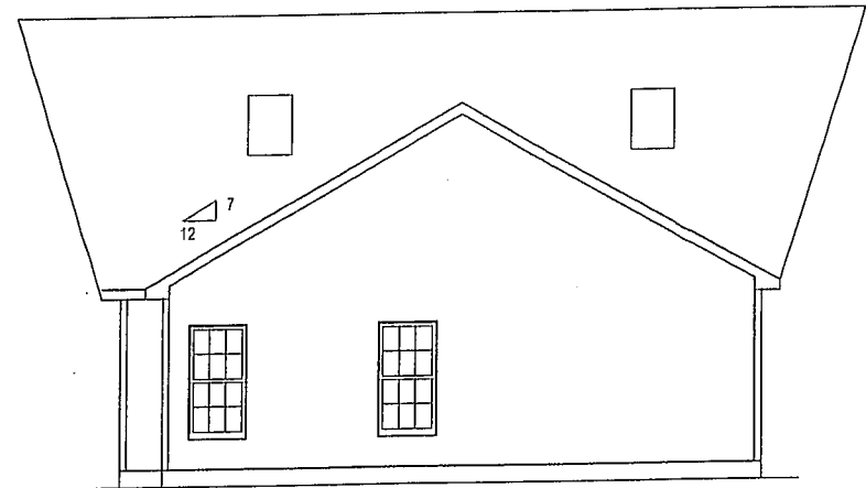
RIGHT VIEW
