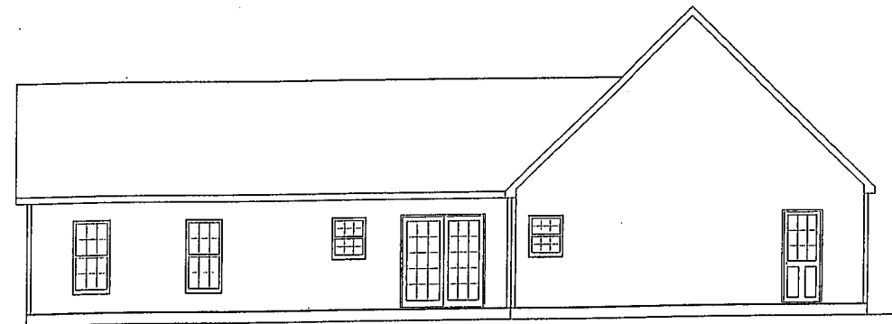
REAR VIEW
