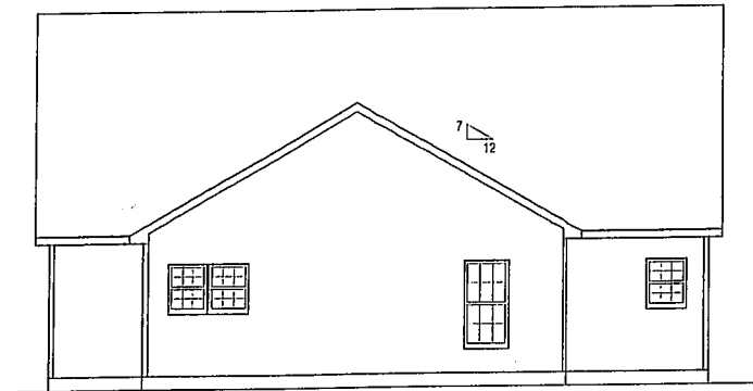
RIGHT VIEW
