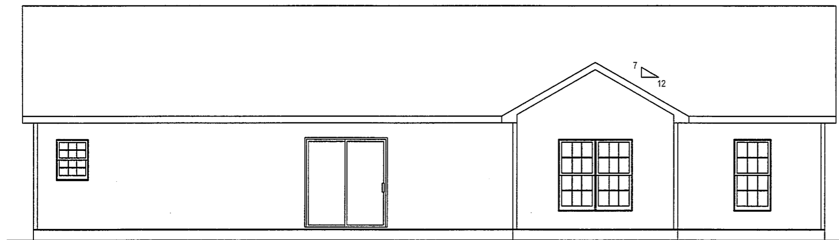
REAR VIEW
