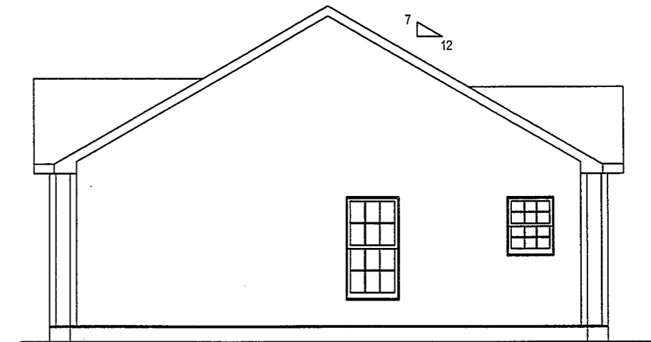
RIGHT VIEW
