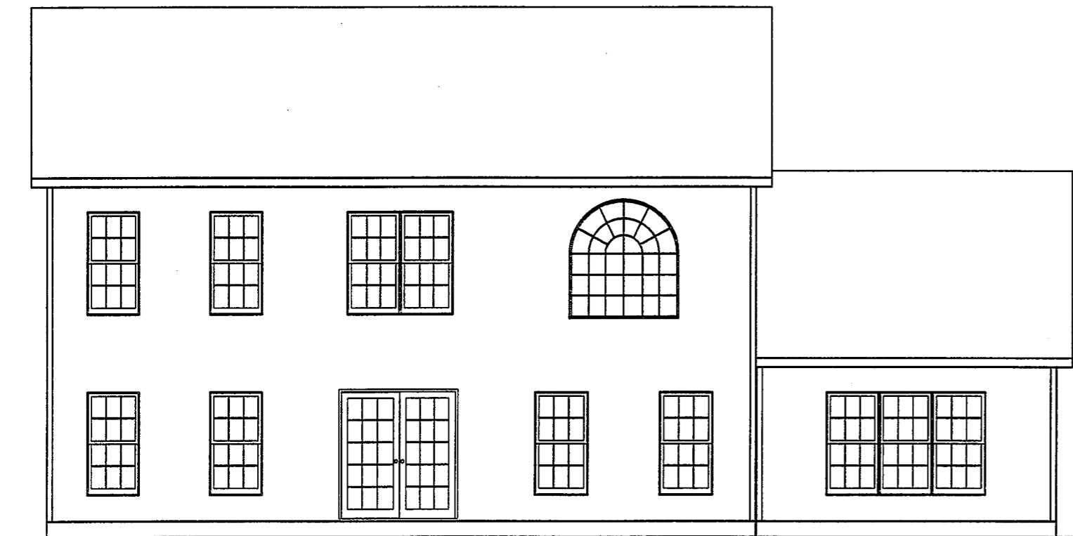
REAR VIEW
