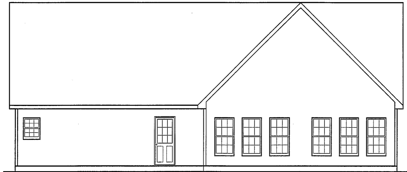
REAR VIEW
