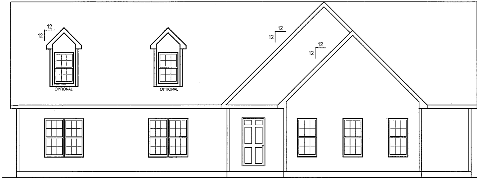
FRONT VIEW
