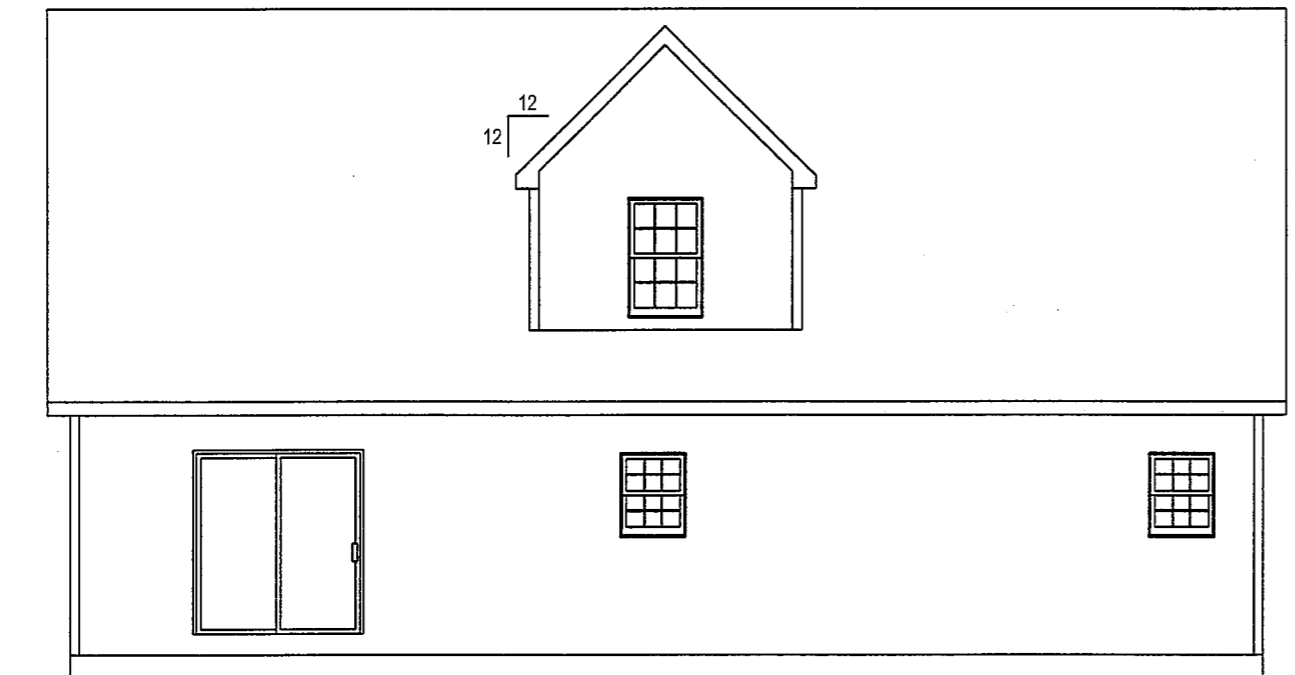
REAR VIEW
