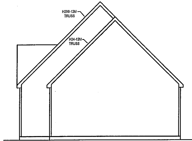
RIGHT VIEW
