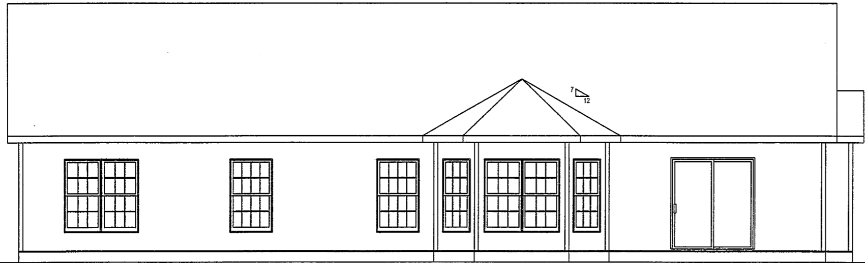
REAR VIEW
